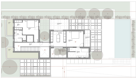
Distribution plan 1st floor
